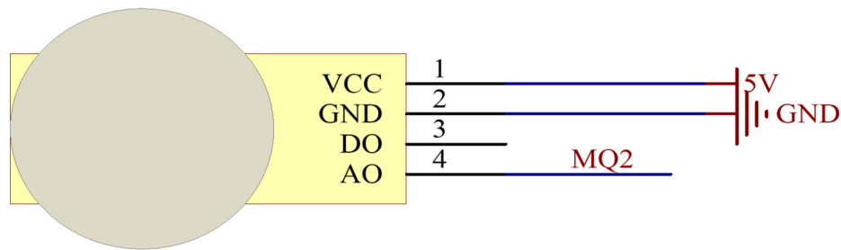
Figure 3-4. Smoke Concentration Sensor Module Interface Circuit
