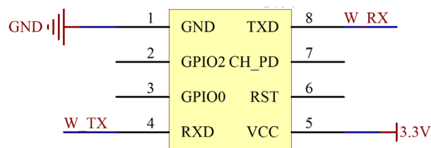
Figure 3-2. WiFi Module
