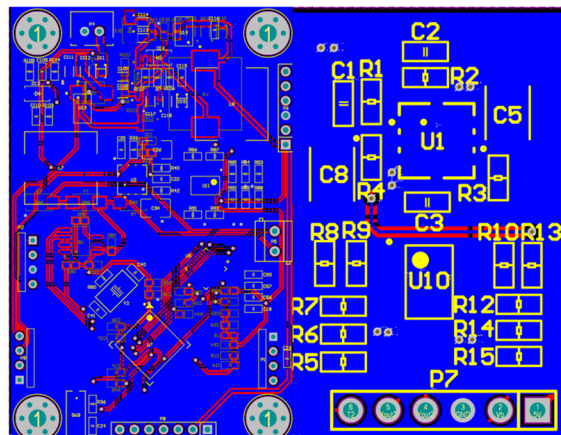
Figure 8. PCB diagram
