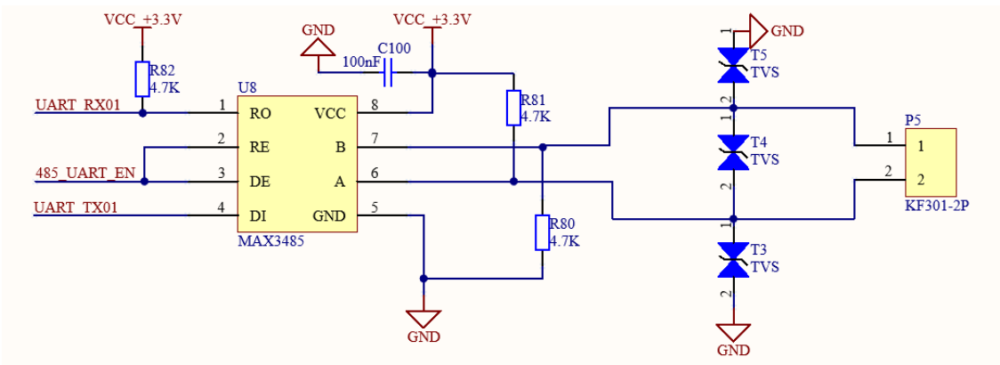
Figure 5. RS485 communication circuit design
