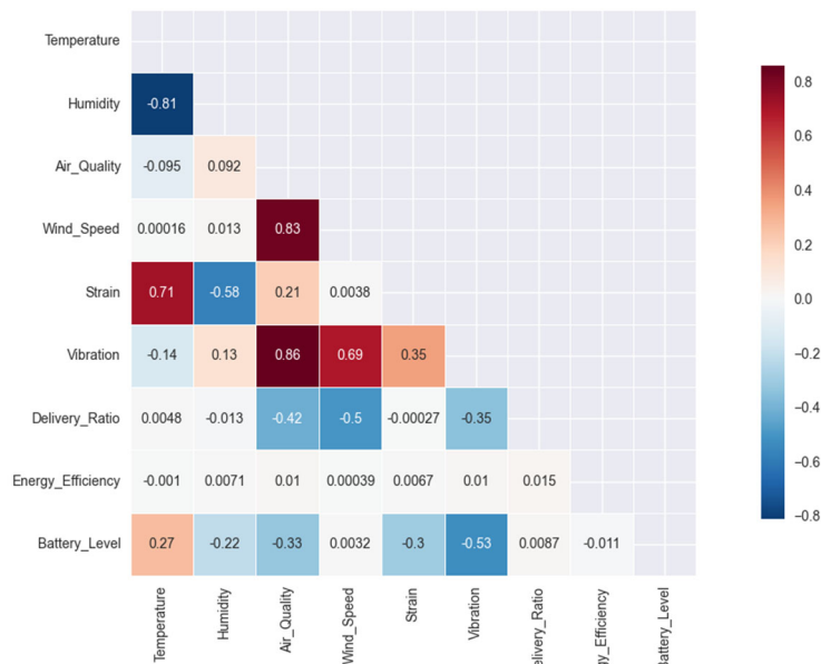
Figure 8. Inter-Parameter Correlation Analysis
