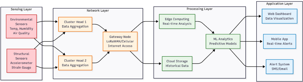
Figure 2. WSN System Architecture
