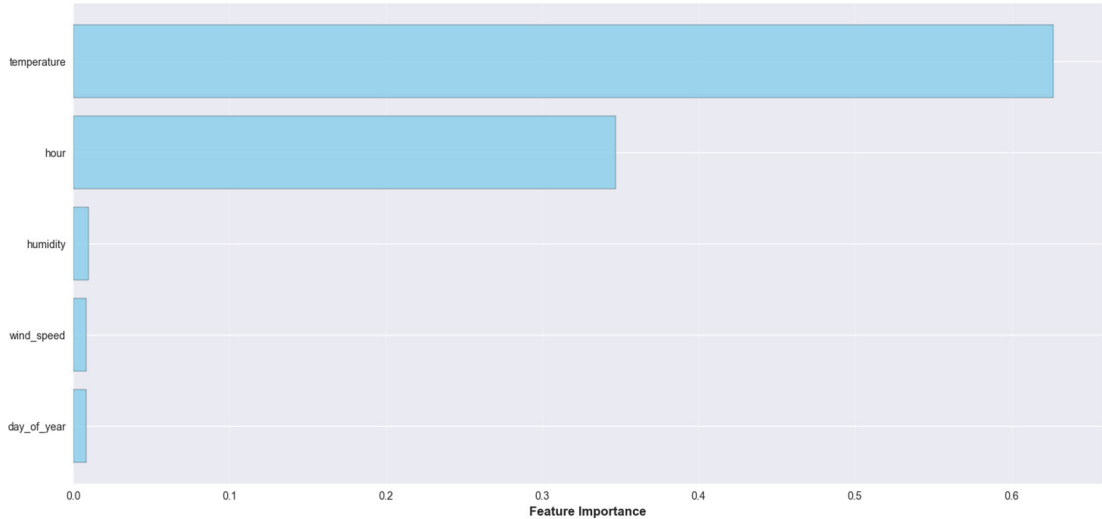
Figure 10. Feature Importance in Strain Prediction Model
