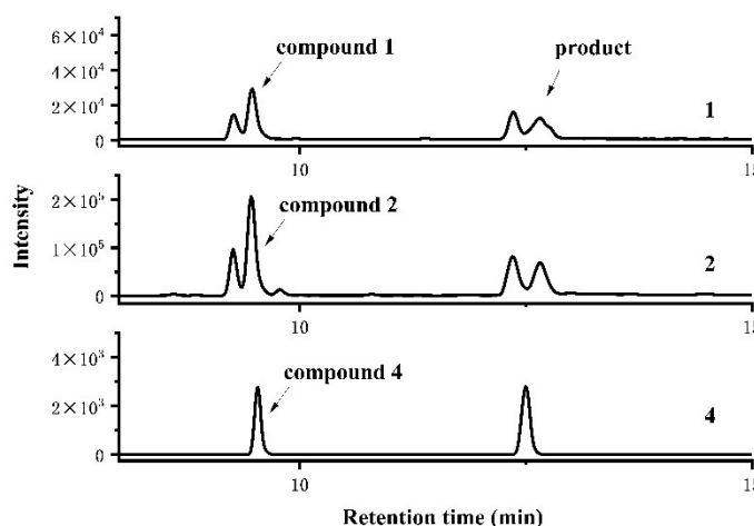
Figure 4. Acid hydrolysis of compounds 1 , 2 and 4
