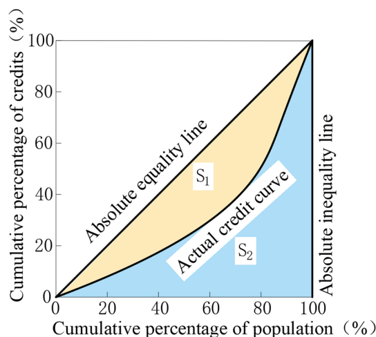
Figure 1. Lorenz curve
