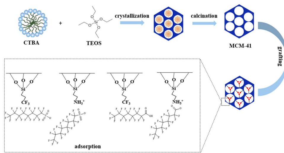
Figure 2. Schematic diagram of material preparation and adsorption.
